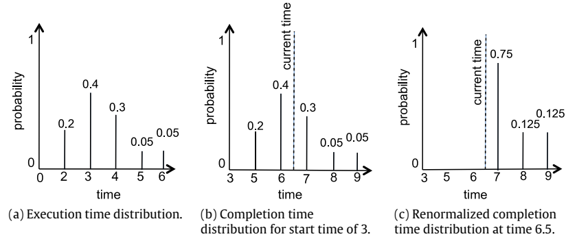
Fig. 2. Execution and completion time distributions for a given task that is being executed in a machine. (a) Execution time distribution of the task. (b) Given that the task started execution at time 3, the completion time distribution for the task after shifting the task execution time distribution. (c) Completion time distribution after renormalizing based on the current time of 6.5 by removing impulses that occur before the current time.
