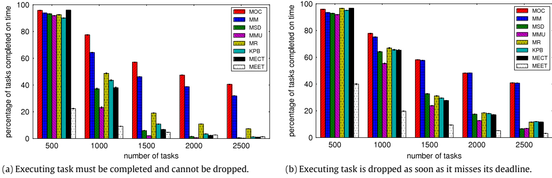
Fig. 10. Percentage of tasks completed on time using immediate and batch mode resource allocation heuristics when the over-subscription level varies in the system. The horizontal axis shows the different number of tasks evaluated. In this experiment, the average task's input data size is 64 MB and the machine queue-size limit is 2. Results are averaged over 100 runs and 95% confidence interval of the results are reported.
