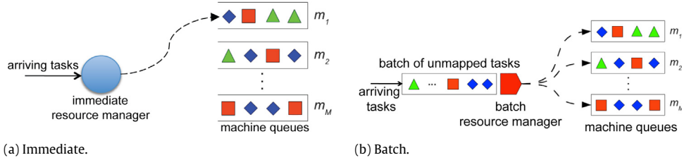
Fig. 1. Dynamic resource allocation that (a) maps arriving tasks to machines immediately upon arrival, and (b) maps a limited number of tasks to each machine and queues the rest of arriving tasks at the resource manager.
