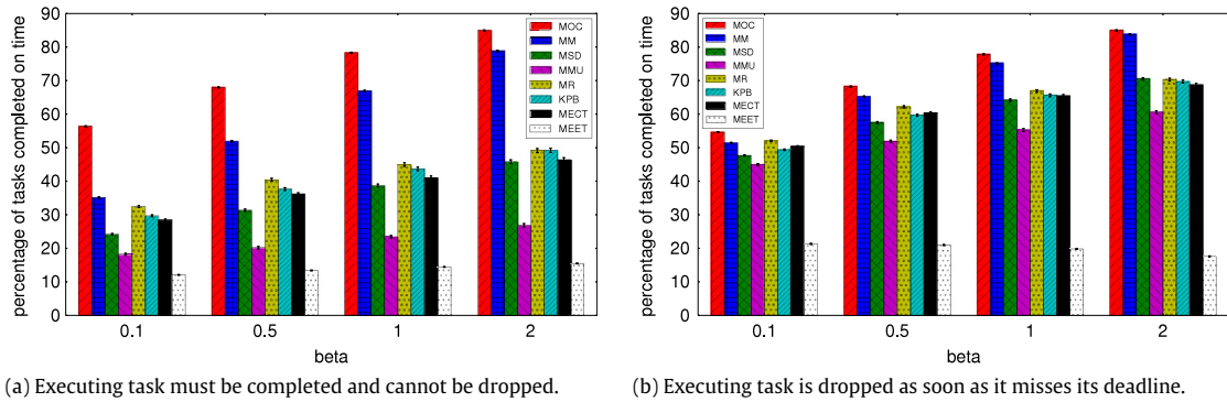
Fig. 11. Percentage of tasks completed on time when immediate and batch mode resource allocation heuristics are applied and the deadline of tasks varies. Higher values of \beta , in the horizontal axis, shows looser deadlines for tasks. In this experiment, the machine queue-size limit is 2, the tasks' average input data size is 64 MB, and 1000 tasks are considered for the evaluation. Results are averaged over 100 runs.
