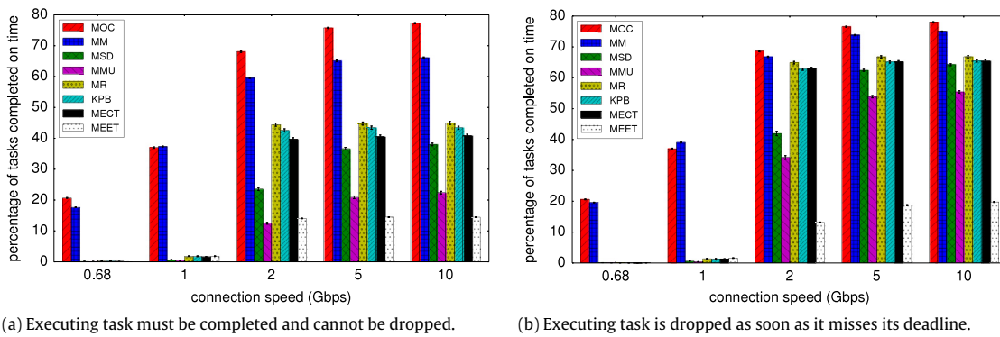
Fig. 9. Percentage of tasks completed on time when immediate and batch mode resource allocation heuristics are applied and the average connection speed in the HC system varies. The horizontal axis shows the different connection speeds evaluated and the vertical axis shows the percentage of tasks that complete on time. In this experiment, the machine queue-size limit is 2, the tasks' average input data size is 1024 MB, and 1000 tasks are considered for the evaluation. Results are averaged over 100 runs.
