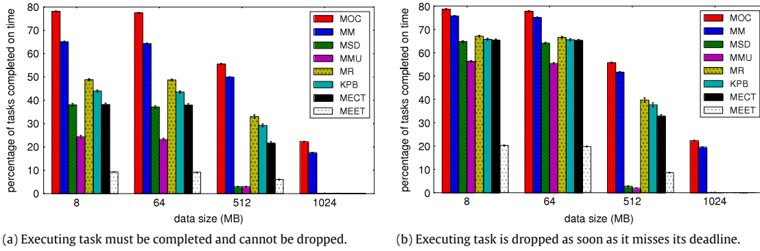
Fig. 8. Percentage of tasks completed on time when immediate and batch mode resource allocation heuristics are applied and average size of tasks' required input data vary. The horizontal axis shows the different input data sizes evaluated. In this experiment, the machine queue-size limit is 2 and 1000 tasks are considered for the evaluation. Results are averaged over 100 runs.
