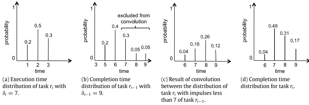
Fig. 3. Completion time distribution for a given task r_i in a system where pending tasks are dropped if they miss their deadlines. (a) Execution time distribution of task r_i with \delta_i = 7 . (b) Completion time distribution of task r_{i-1} with \delta_{i-1} = 9 . (c) Distribution resulted from convolving impulses of task r_i with impulses less than time 7 of task r_{i-1} . (d) Completion time distribution for task r_i ; obtained from adding impulses greater than or equal to 7 in completion time pmf of task r_{i-1} in Fig. 3(b), for which task r_i is dropped and has execution time zero, with the distribution in Fig. 3(c).
