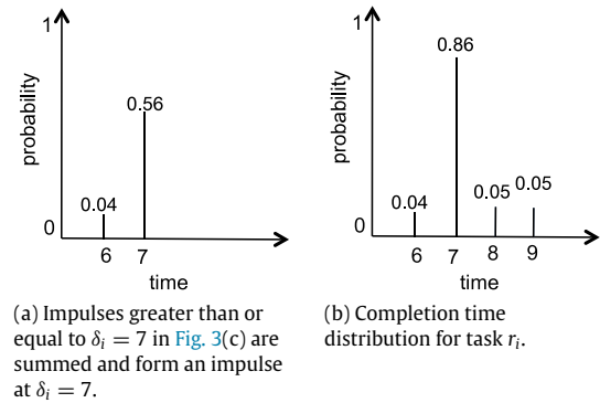
Fig. 4. Completion time distribution of task r_i in a system where the currently executing task is dropped as soon as it misses its deadline. (a) After convolving the distribution of task r_i with impulses less than time 7 in the distribution of task r_{i-1} in Fig. 3(c), impulses greater than or equal to the deadline of task r_i in the resulting distribution are summed and form an impulse at \delta_i = 7 . (b) Completion time distribution for task r_i ; obtained from adding the distribution in Fig. 4(a) with the excluded impulses of task r_{i-1} in Fig. 3(b), for which task r_i is dropped and has execution time zero.
